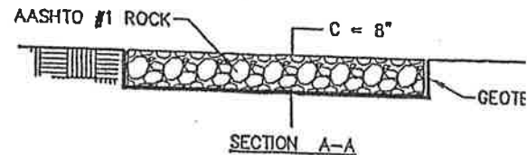
CONSTRUCTION ENTRANCE
