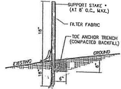
STANDARD SILT FENCE DETAIL NOT TO SCALE
