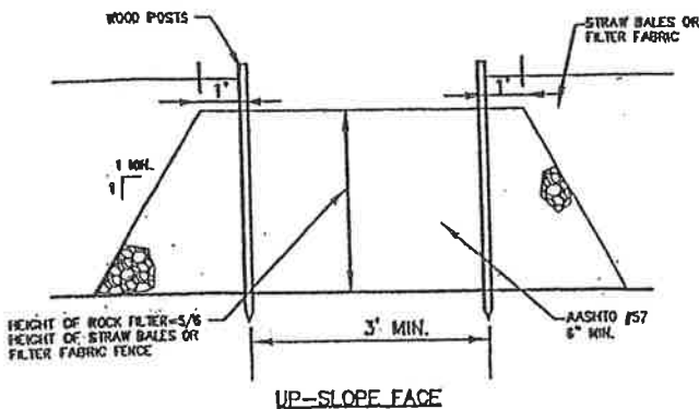
ROCK FILTER OUTLET DETAIL
