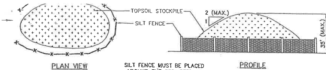
PLAN VIEW
