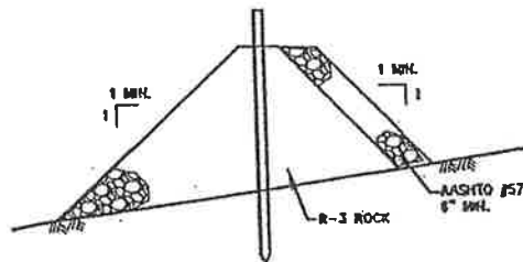
OUTLET CROSS SECTION
